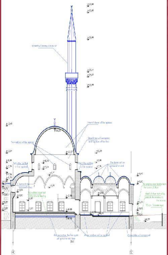
SECTION 2-2
